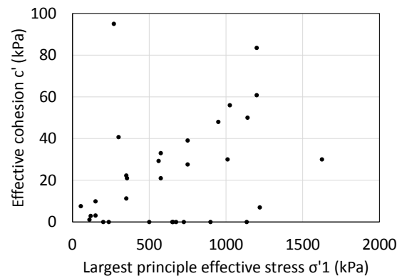
Figure 5: Effective cohesion from previous triaxial tests
