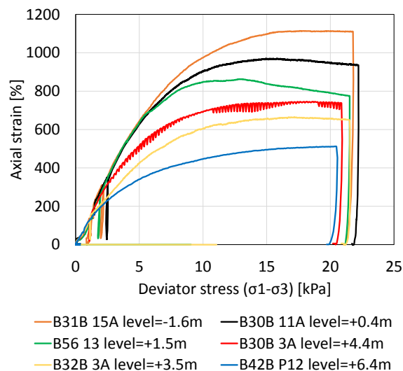
Figure 7: Stress strain curves from CAU tests
