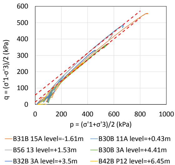
Figure 9: Effective stress path from CAU tests
